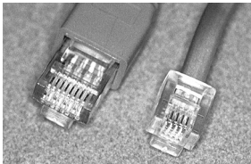
FIGURE 221. RJ-45 connector ( left ) and RJ-11 connector ( right )
