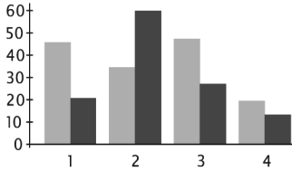
FIGURE 27. Bar graph
