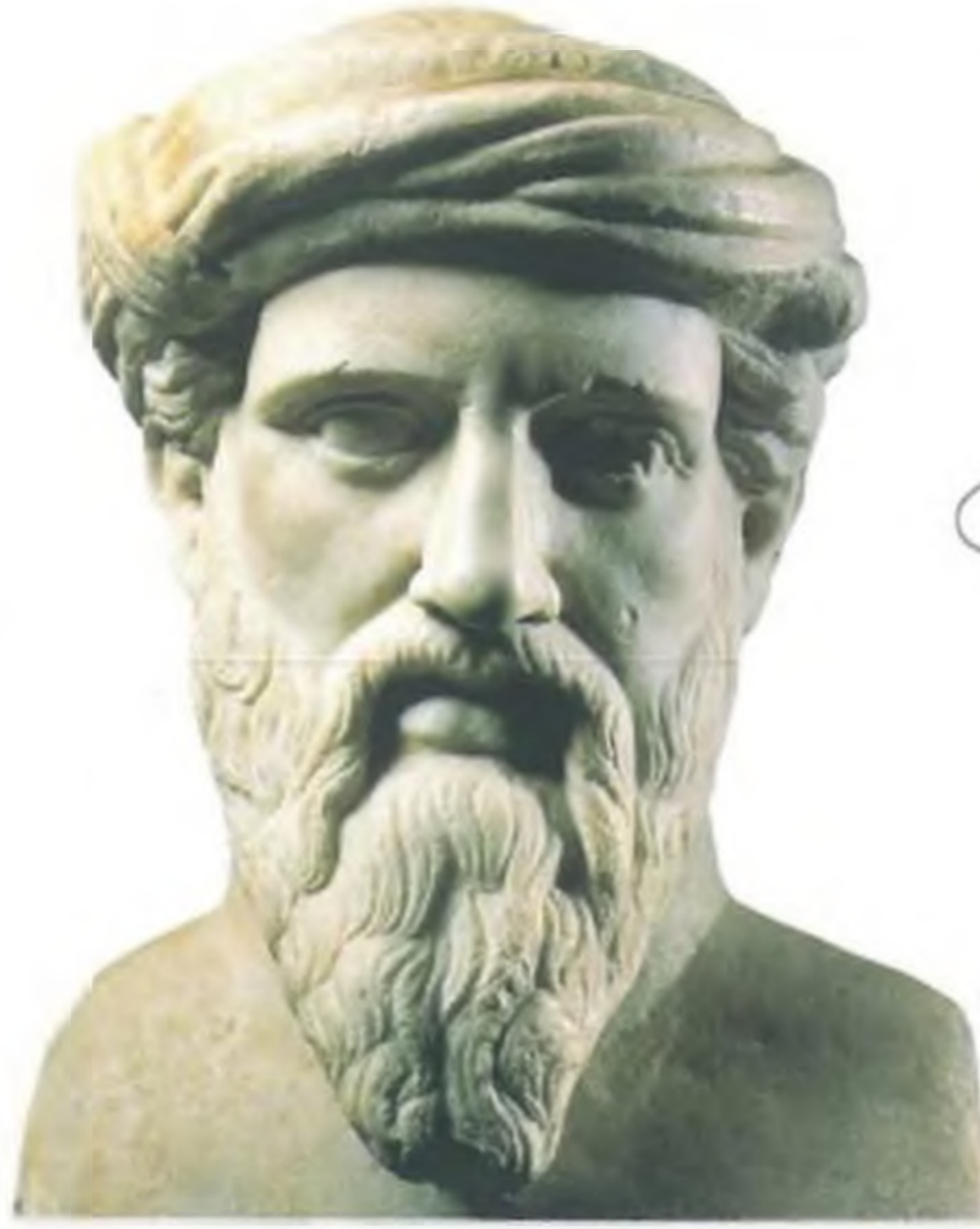
PYTHAGORAS
