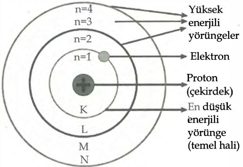
Bohr atom modeli
